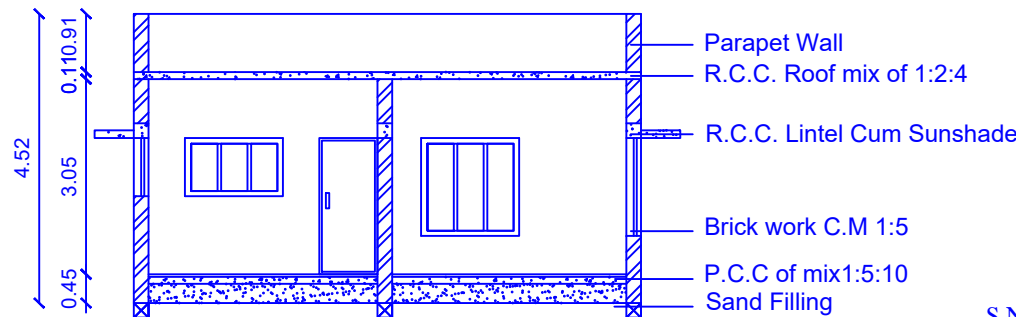
SECTION ON RS
