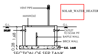
SECTION OF SEPT.TANK
