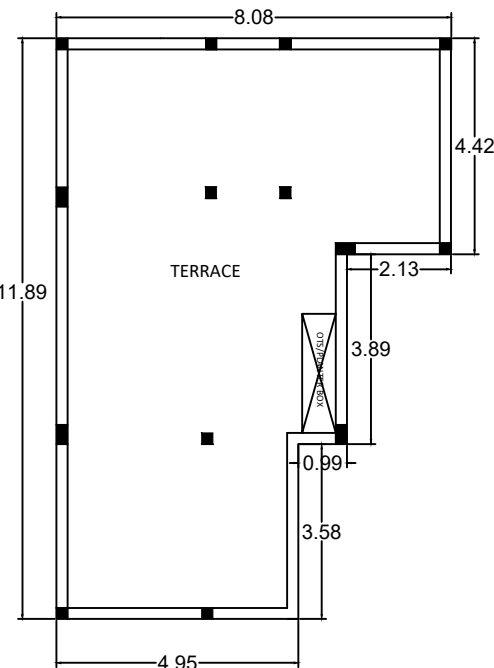
TERRACE FLOOR PLAN SCALE 1:50
