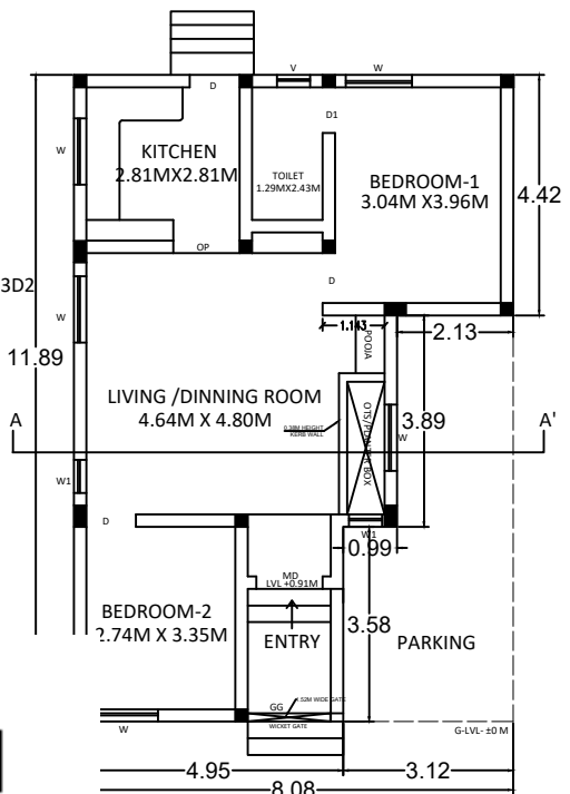
POSED GROUND FLOOR PLAN SCALE 1:50
