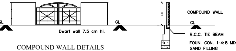
SECTION
