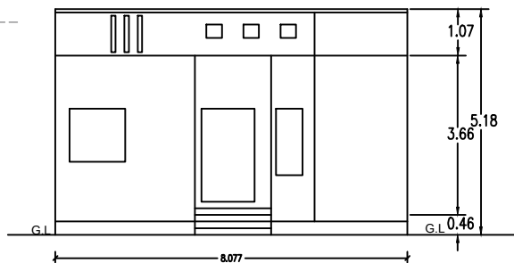
FRONT ELEVATION SCALE 1:50
