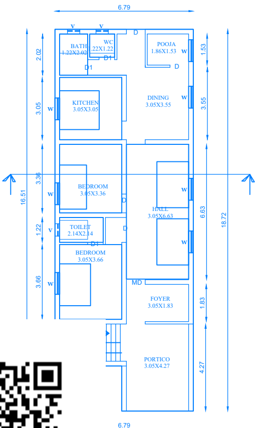
D FLOOR PLAN
