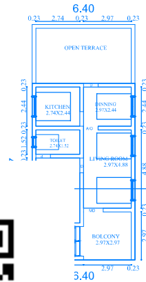
FLOOR PLAN
