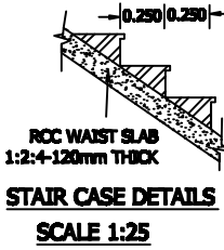
STAIR CASE DETAILS SCALE 1:25
