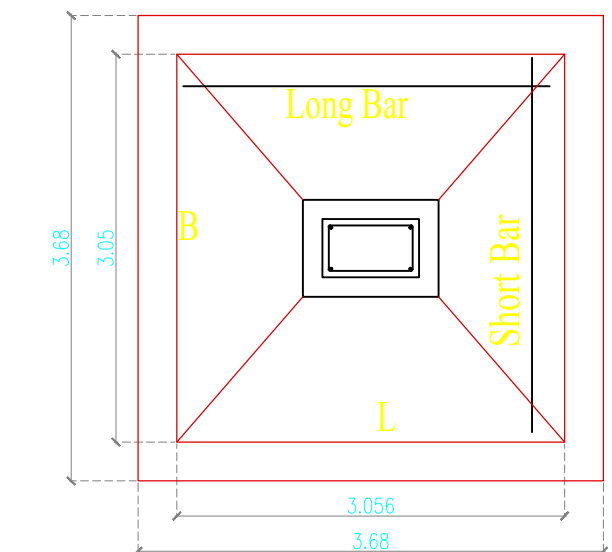
PLAN OF FOOTING
