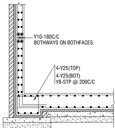
TYPICAL RAFT DETAIL
