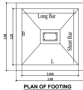
PLAN OF FOOTING
