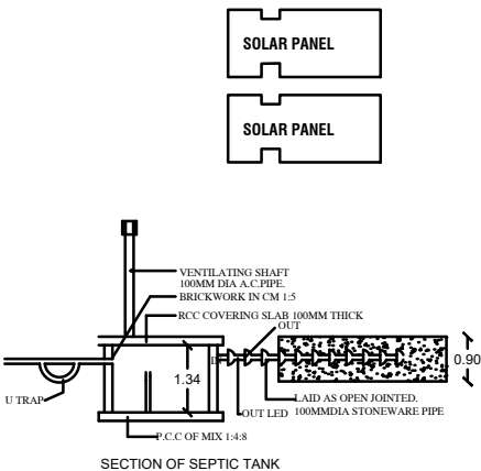
SECTION OF SEPTIC TANK
