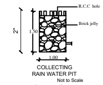
COLLECTING RAIN WATER PIT Not to Scale RWH_CAPACITY_L=1000 LTRS
