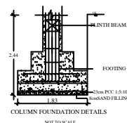
COLUMN FOUNDATION DETAILS NOT TO SCALE
