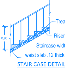
STAIR CASE DETAIL
