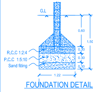
FOUNDATION DETAIL
