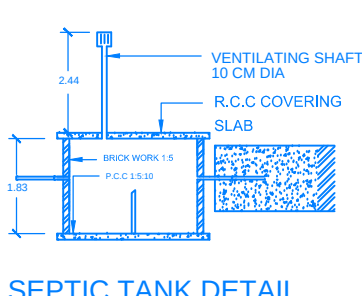
SEPTIC TANK DETAIL
