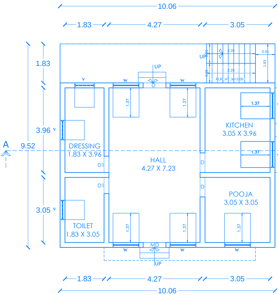
COR PLAN
