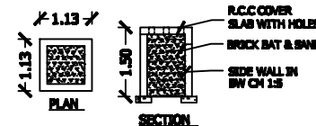
RAIN WATER HARVESTING PIT
