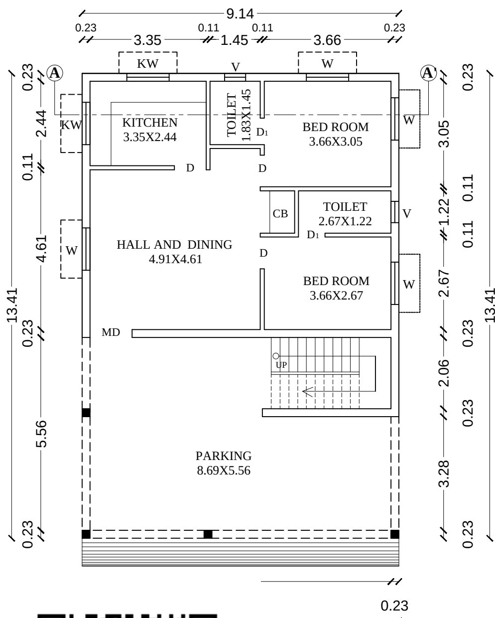
FLOOR PLAN
