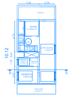
6.70 SECOND FLOOR PLAN
