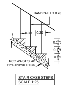
STAIR CASE STEPS SCALE 1:25
