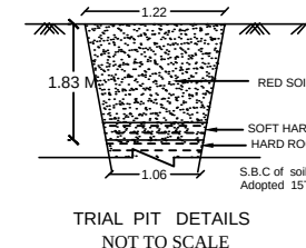
TRIAL PIT DETAILS NOT TO SCALE
