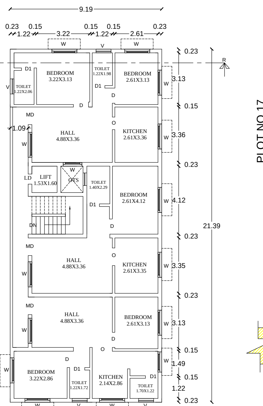
PRO- SECOND FLOOR PLAN
