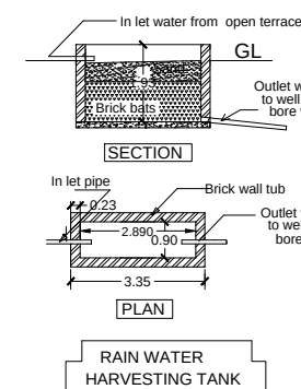
RAIN WATER HARVESTING TANK
