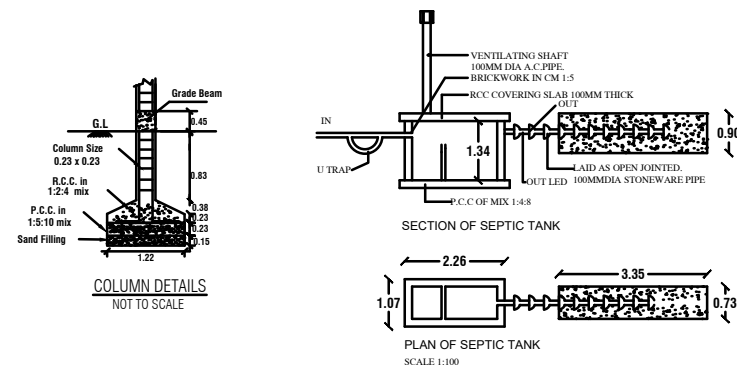
SCALE 1:100
