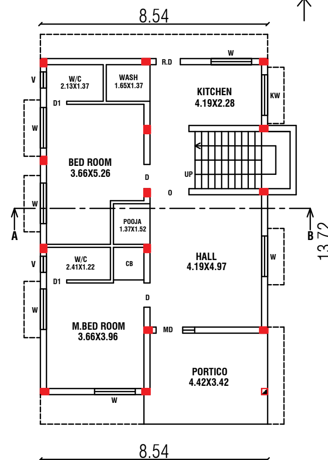
EXI.GROUND FLOOR PLAN
