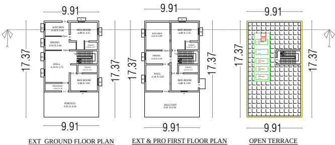
EXT GROUND FLOOR PLAN
