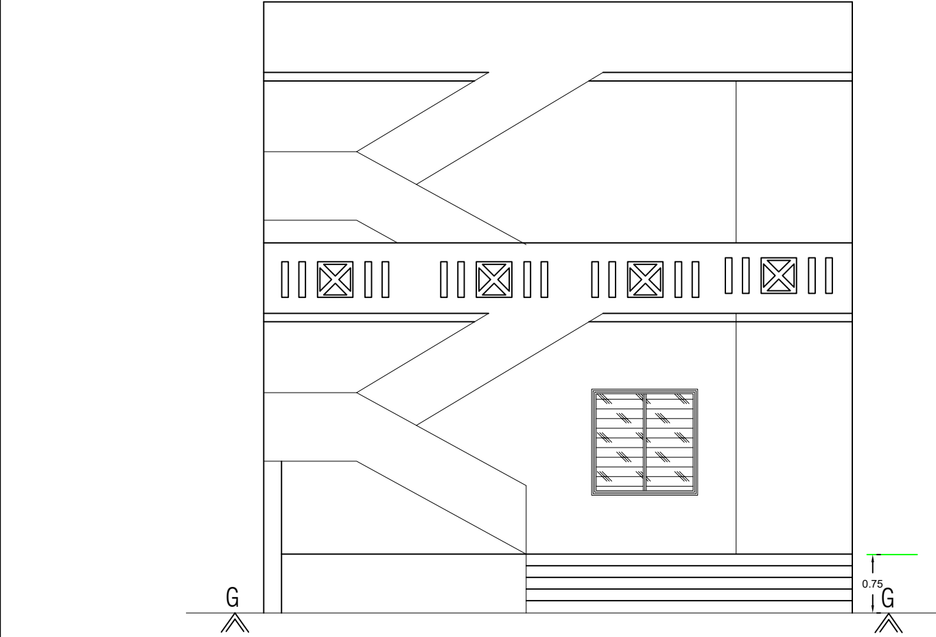
FRONT ELEVATION
