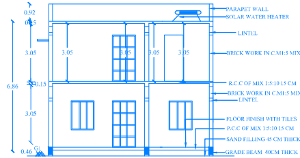
SECTION-AA1
