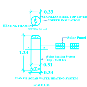
SCALE 1:50
