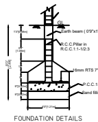
FOUNDATION DETAILS
