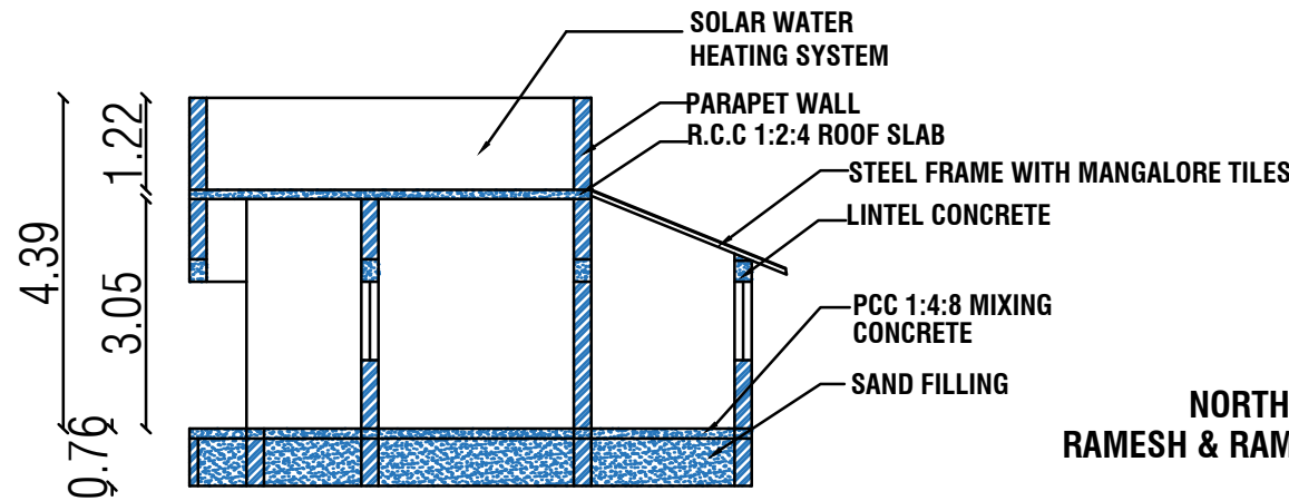
SECTION NO - "AB"
