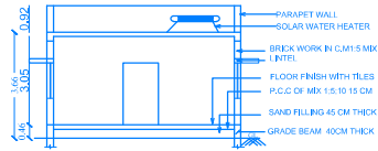
SECTION-AB
