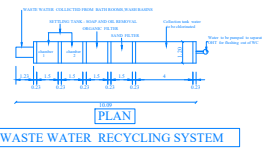
PLAN WASTE WATER RECYCLING SYSTEM
