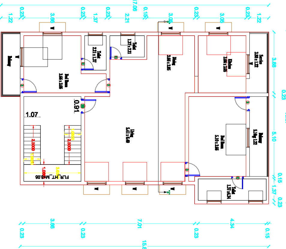
EXISTING FIRST FLOOR
