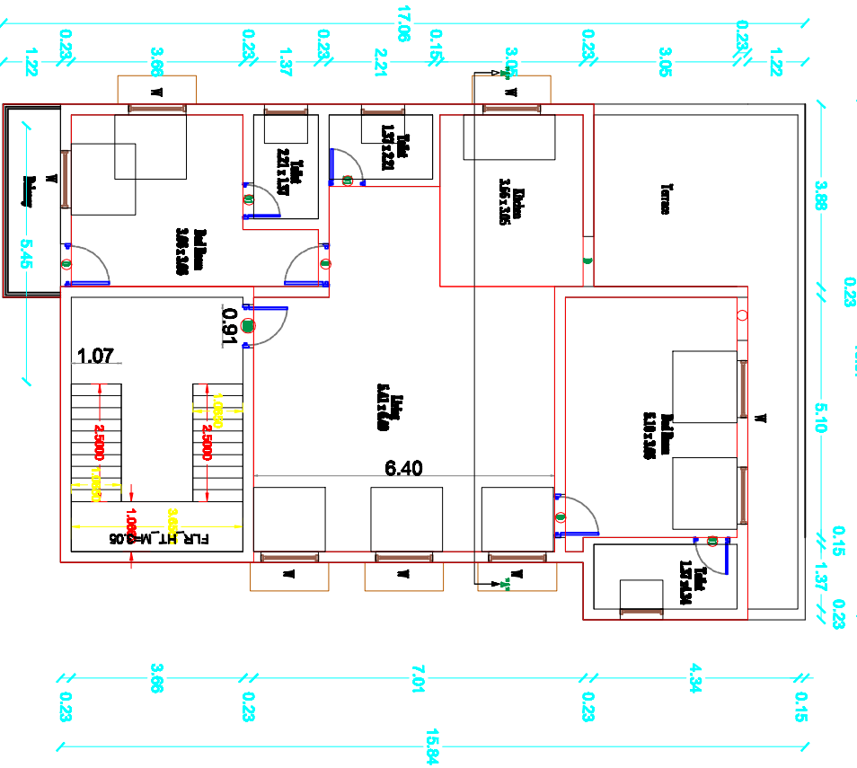
PROPOSED SECOND FLOOR
