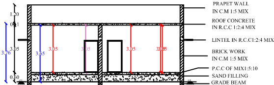
SECTION - XX
