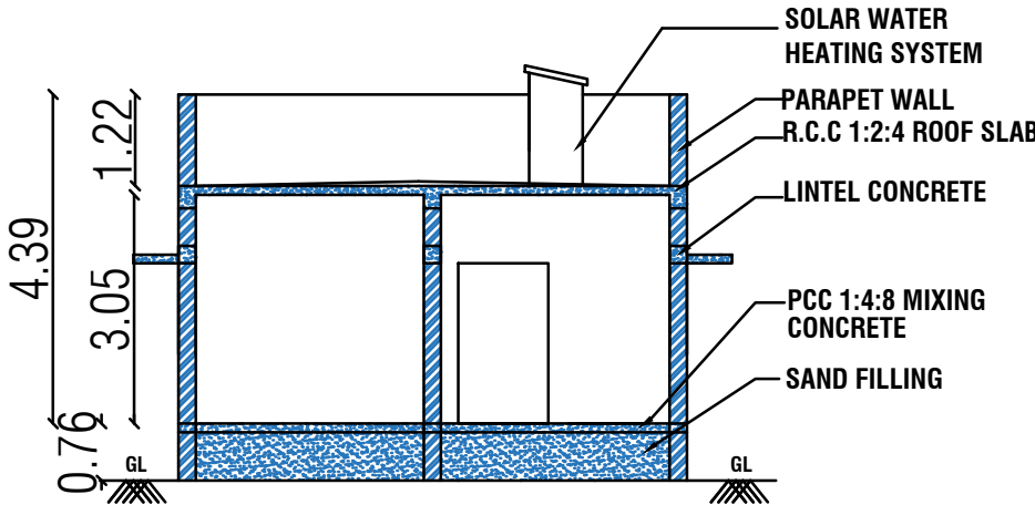
SECTION NO -"AB"
