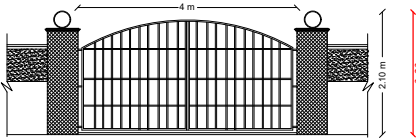
COMPOUND GATE (NOT TO SCALE)
