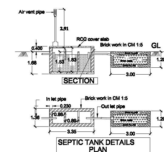
SEPTIC TANK DETAILS PLAN
