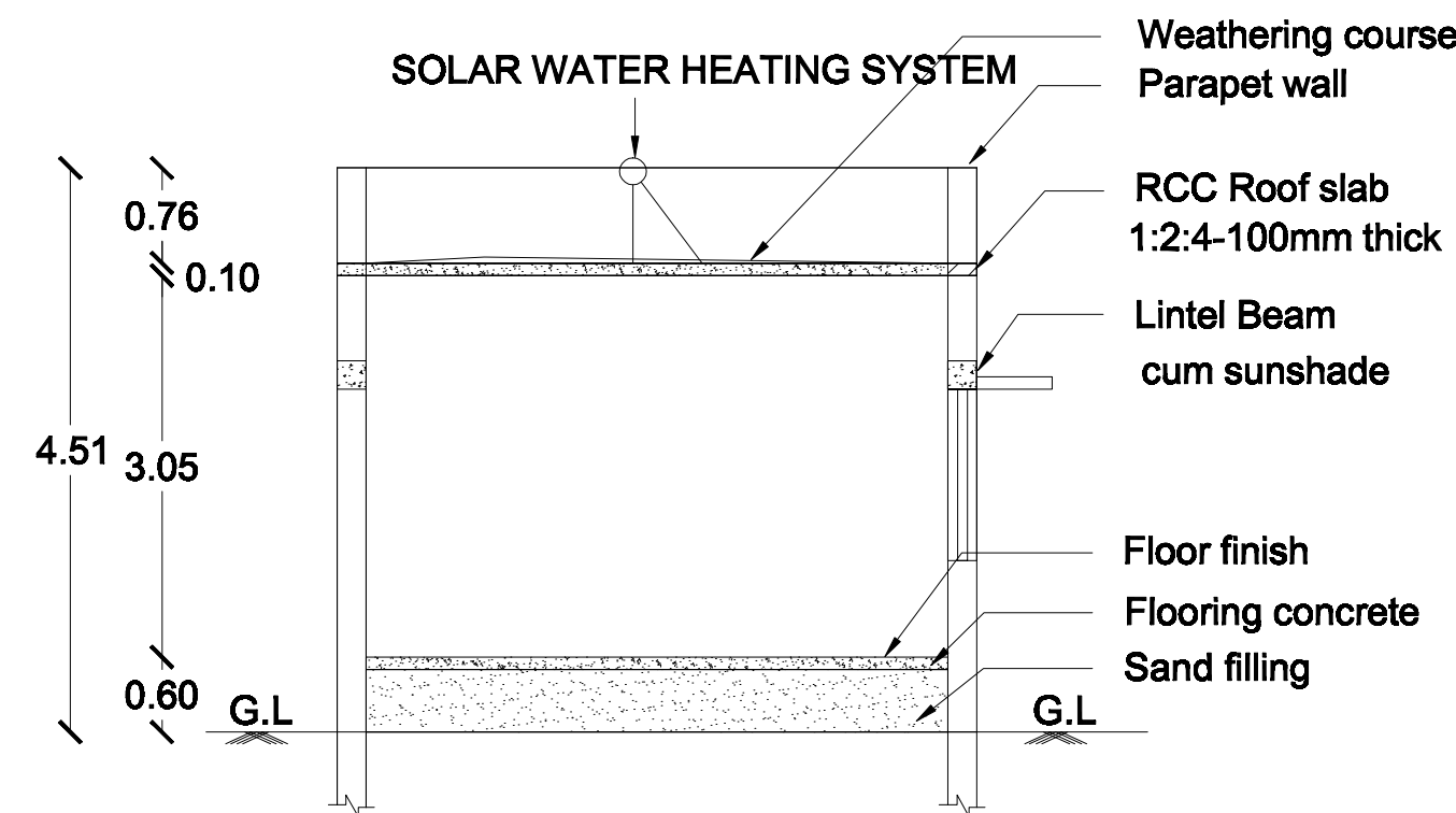
SECTION ON MK
