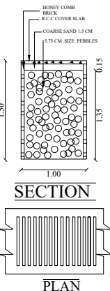
RAIN WATER HARVESTING PERCOLATION BED
