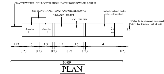
WASTE WATER RECYCLING SYSTEM PLAN
