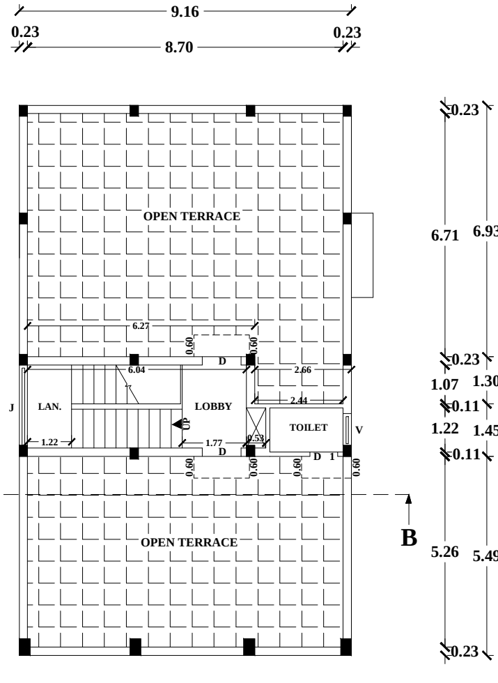
HEAD ROOM FLOOR PLAN
