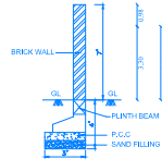
COMPOUND WALL DETAIL
