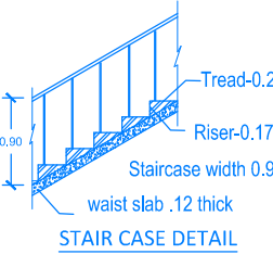
STAIR CASE DETAIL
