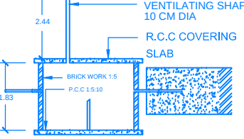
SEPTIC TANK DETAIL
