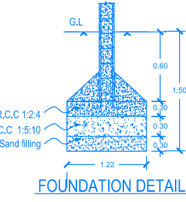
FOUNDATION DETAIL
