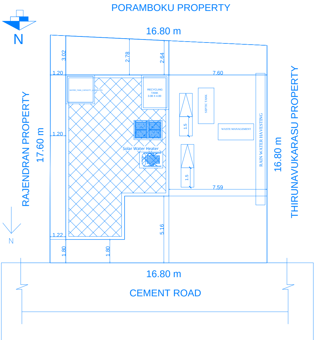
SITE PLAN
