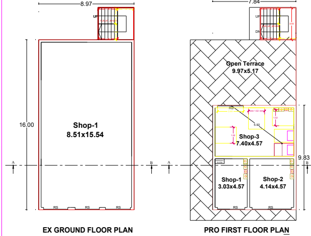
EX GROUND FLOOR PLAN
