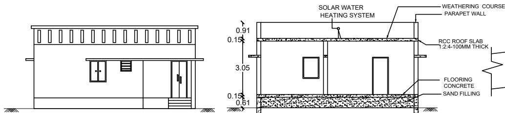
SECTION NP
