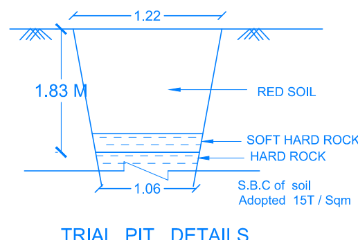
TRIAL PIT DETAILS NOT TO SCALE
