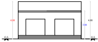
FRONT ELEVATION
