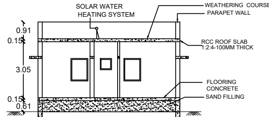
SECTION NP
