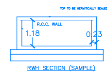
RWH_SECTION (SAMPLE)
