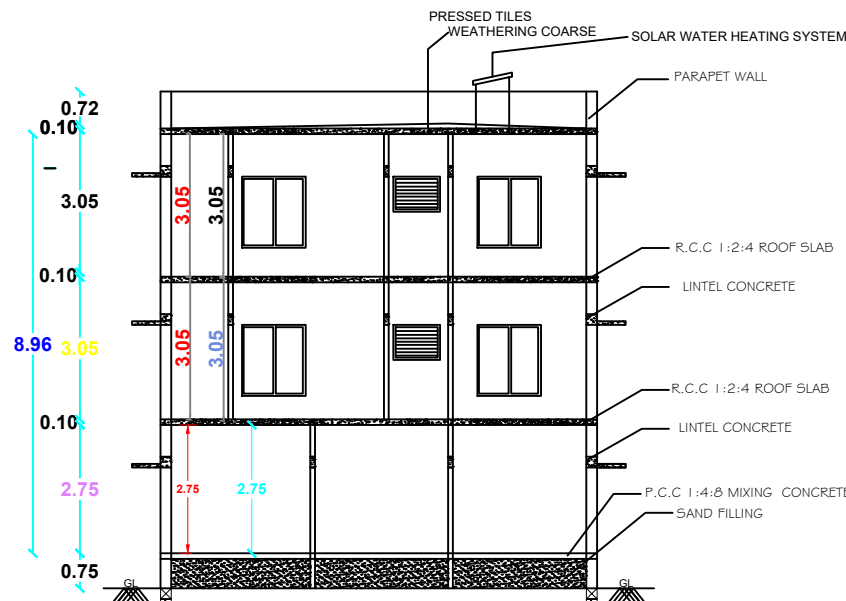
SECTION ON-'SS'
