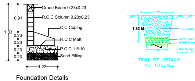
Foundation Details
