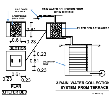
RAIN WATER COLLECTION SYSTEM FROM TERRACE
