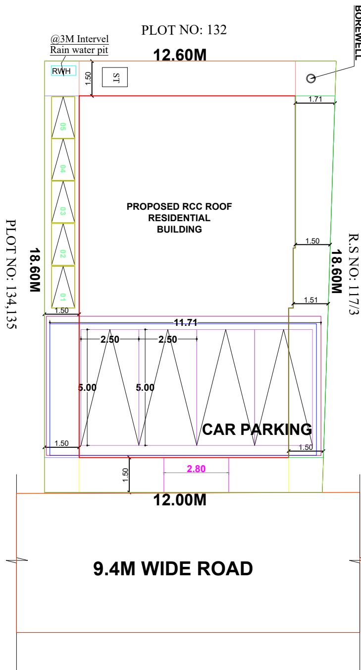
SITE PLAN (1:100)
