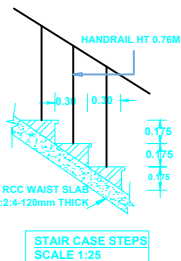
STAIR CASE STEPS
