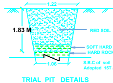
TRIAL PIT DETAILS
