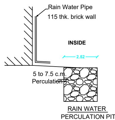
RAIN WATER PERCUSSION PIT
