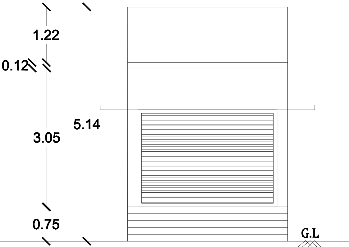
FRONT ELEVATION
