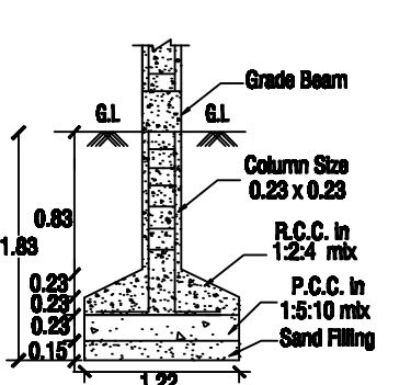
COLUMN DETAIL
