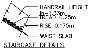
STAIRCASE DETAILS
