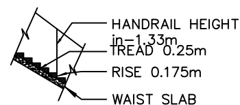
STAIRCASE DETAILS
