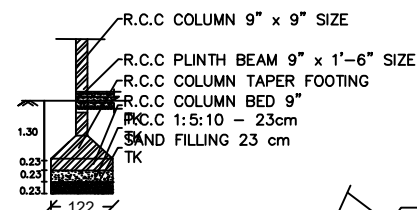
SECTION
