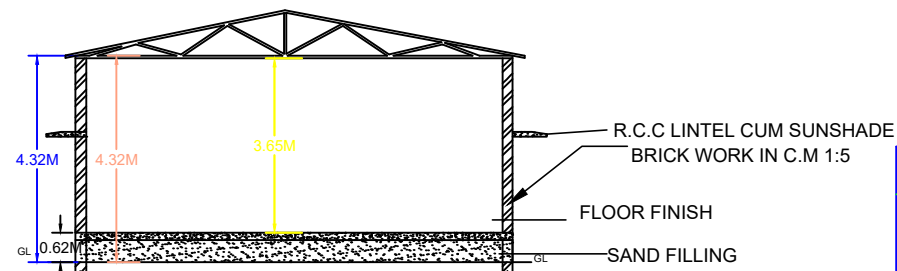
SECTION ON XX
