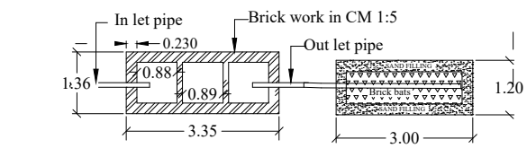
SEPTIC TANK DETAILS PLAN
