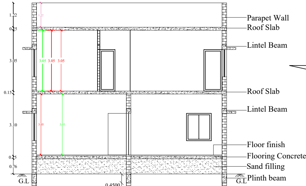
SECTION ON HH
