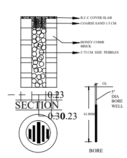
PLAN RAIN WATER HARVESTING 1.PERCOLATION PIT
