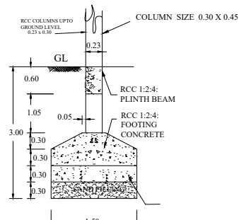
FOUNDATION DETAILS Not to Scale
