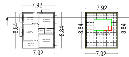
PRO.GROUND FLOOR PLAN
