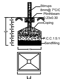
Foundation Details
