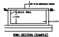
RWH SECTION (SAMPLE) RWH_CAPACITY_L = 2000LTRS
