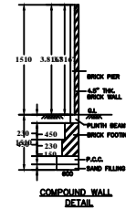
COMPOUND WALL DETAIL
