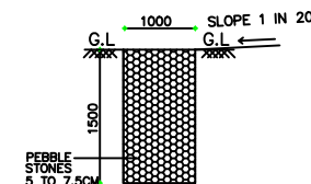
SECTION OF PEBBLE TRENCH SCALE : 1 : = 100
