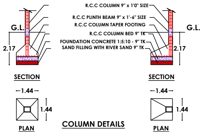
COLUMN DETAILS
