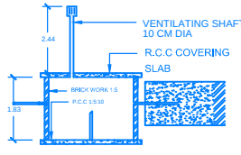
SEPTIC TANK DETAIL
