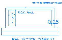
RWL SECTION (SAMPLE)
