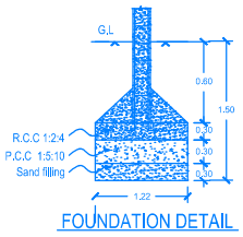
FOUNDATION DETAIL
