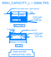
RAIN WATER HARVESTING TANK
