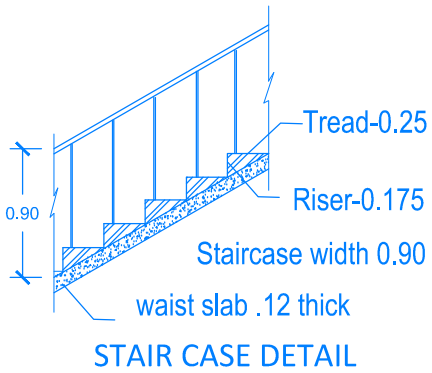
STAIR CASE DETAIL
