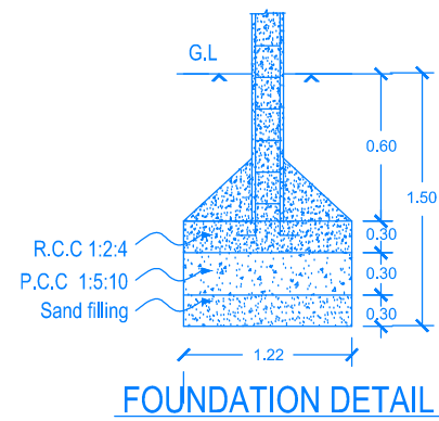
FOUNDATION DETAIL
