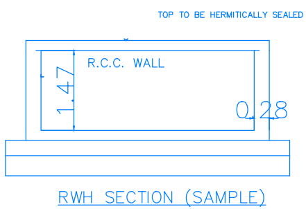
RWH_SECTION (SAMPLE)
