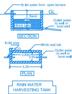
RAIN WATER HARVESTING TANK
